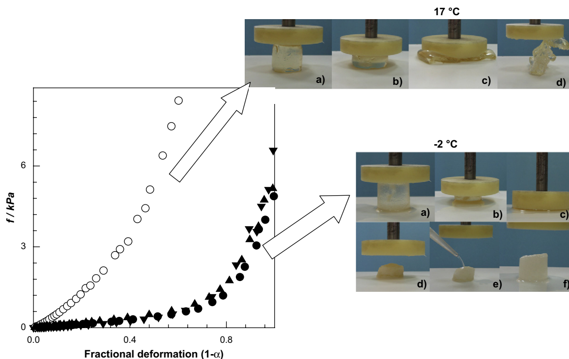
Fig. 12. Typical stress–strain data of PIB gels as the dependence of f on 1 - \alpha . \text{S}_2\text{Cl}_2 = 5.7\% . Reaction time = 3 days. Freezing rate = slow. T_{prep} = 17^\circ\text{C} ( \circ ), -2^\circ\text{C} ( \blacktriangle ), -10^\circ\text{C} ( \bullet ), and -18^\circ\text{C} ( \blacktriangledown ). Photographs show the gels formed at 17^\circ\text{C} (upper panel) and at -2^\circ\text{C} (lower panel) during the compression test. After compression of -2^\circ\text{C} gel, addition of toluene converts the gel back to its initial state.
