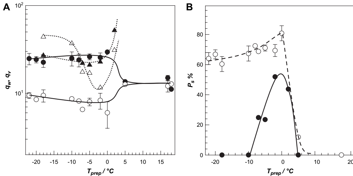
Fig. 5. (A): The equilibrium weight ( q_w , filled symbols) and the equilibrium volume swelling ratios ( q_v , open symbols) of PIB gels in toluene shown as a function of T_{prep} . Reaction time = 1 day (triangles) and 3 days (circles). (B): The swollen state porosities P_s of the organogels are calculated by using Eq. (4). Reaction time = 1 day (filled symbols, solid curve) and 3 days (open symbols, dashed curve).
