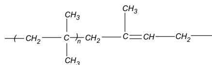
Scheme 1. The structure of butyl rubber.
