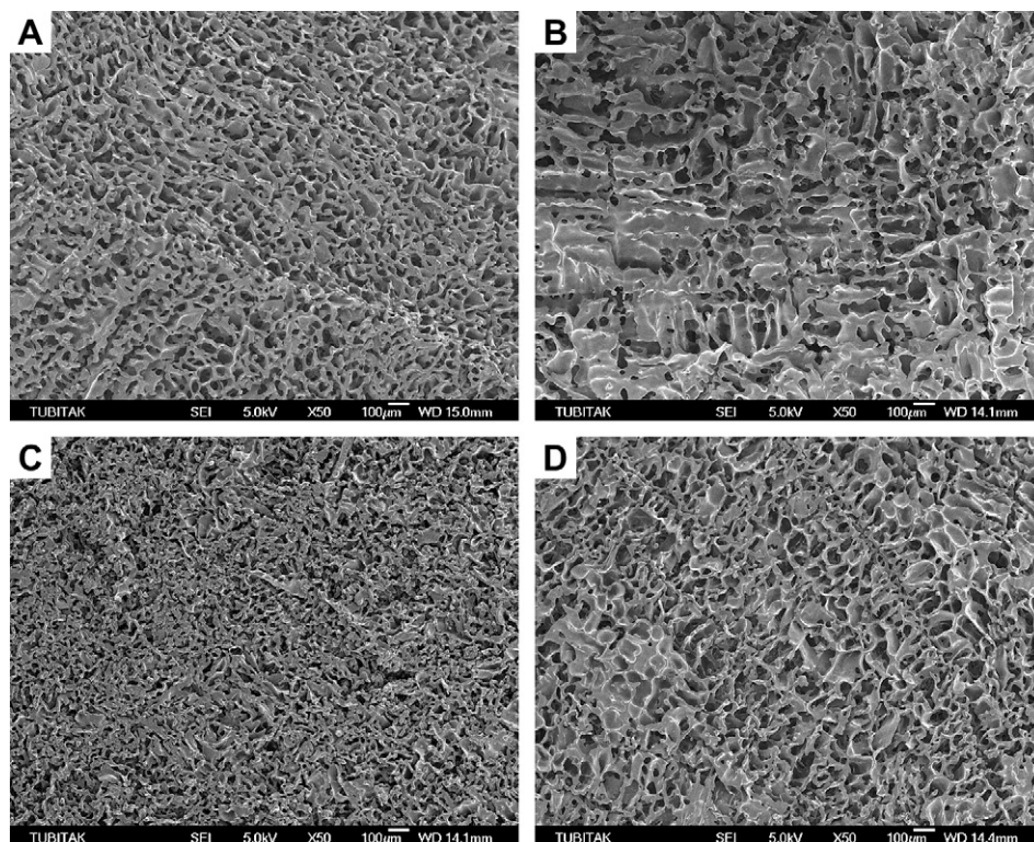
Fig. 7. SEM of PIB networks formed T_{\text{prep}} = -2 (A, B) and -10 °C (C, D). Freezing rate = fast (left panel), slow (right panel). Reaction time = 3 days. S_2Cl_2 = 5.7\% . The scaling bars are 100 \mu\text{m} . Magnification = 50 \times .
