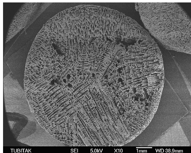
Fig. 1. SEM of PIB network formed in cyclohexane at T_{prep} = -2 °C. Reaction time = 24 h. \text{S}_2\text{Cl}_2 = 5.7\% . The scaling bar is 1 mm. Magnification = 10\times .
