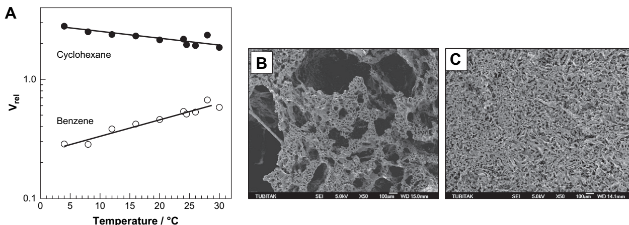
Fig. 8. (A) Normalized volume swelling ratio V_{\text{rel}} of PIB gel in cyclohexane (filled symbols) and in benzene (open symbols) shown as a function of the temperature. The gel was prepared at 17 °C in cyclohexane. Reaction time = 3 days. S_2Cl_2 = 5.7\% . (B) SEM images of PIB networks formed at T_{\text{prep}} = -10 °C in benzene (B) and in cyclohexane (C) under fast freezing condition. Reaction time = 3 days. S_2Cl_2 = 5.7\% . The scaling bars are 100 \mu\text{m} . Magnification = 50 \times .
