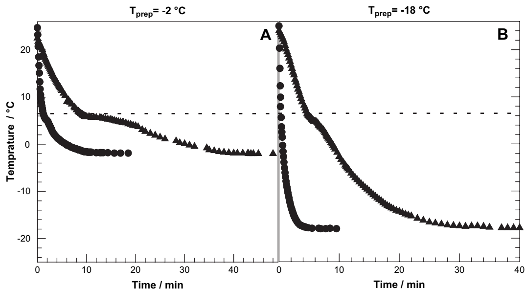
Fig. 6. Cooling profiles of the reaction solutions of 10 mL volume to attain T_{prep} = -2 (A) and -18 °C (B) under slow (triangles) and fast cooling (circles) conditions.
