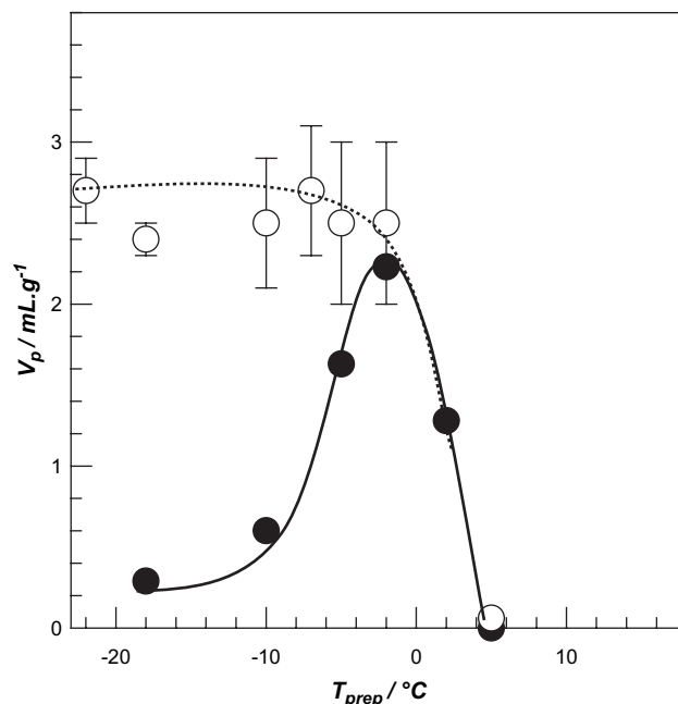
Fig. 4. The total volume of the pores V_p in PIB gels estimated from the uptake of methanol by the gel networks plotted against the temperature T_{\text{prep}} . Reaction time = 1 day (filled symbols, solid curve) and 3 days (open symbols, dashed curve).
