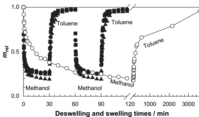
Fig. 10. The normalized mass m_{rel} of PIB gels shown as a function of the time of deswelling in methanol and re-swelling in toluene. S_2Cl_2 = 5.7\% . Reaction time = 3 days. Freezing rate = slow. T_{prep} = -2\text{ }^\circ\text{C} ( \blacktriangle ), -10\text{ }^\circ\text{C} ( \bullet ), -18\text{ }^\circ\text{C} ( \blacksquare ), and 17\text{ }^\circ\text{C} ( \circ ).
