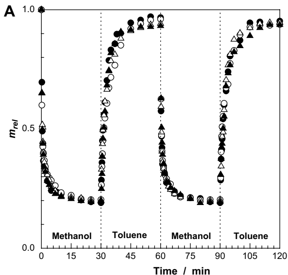
Fig. 9. (A) The normalized mass m_{rel} of PIB gels shown as a function of the time of deswelling in methanol and re-swelling in toluene. S_2Cl_2 = 5.7\% . T_{prep} = -2\text{ }^\circ\text{C} . Reaction time = 1 day, freezing rate = slow ( \circ ), fast ( \Delta ). Reaction time = 3 days, freezing rate = slow ( \bullet ), fast ( \blacktriangle ). (B) Optical microscopy image of a PIB gel sample prepared at -2\text{ }^\circ\text{C} under fast freezing. S_2Cl_2 = 5.7\% . Reaction time = 1 day.
