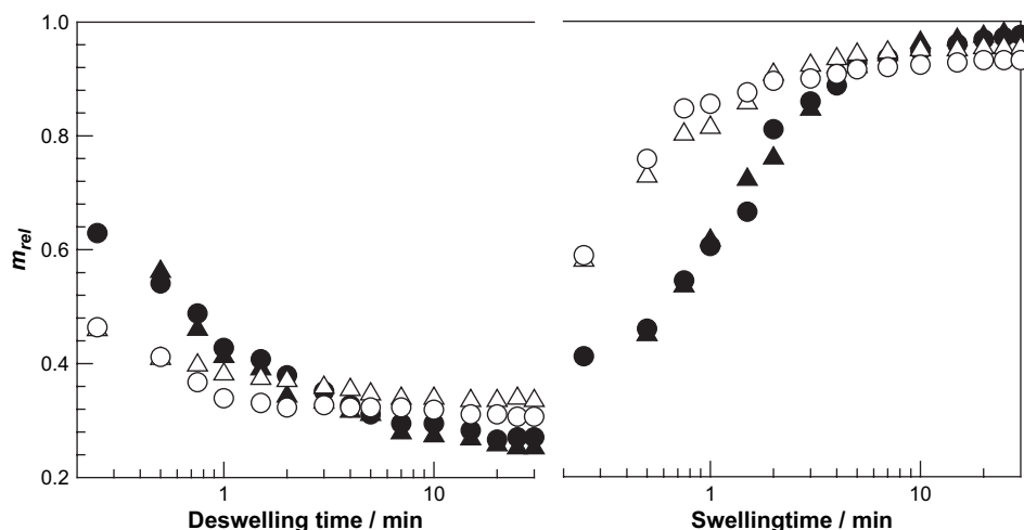
Fig. 11. The normalized mass m_{rel} of PIB gels shown as a function of the time of deswelling in methanol and re-swelling in toluene. \text{S}_2\text{Cl}_2 = 5.7\% . Reaction time = 3 days. Freezing rate = slow. T_{prep} = -10^\circ\text{C} ( \circ , \bullet ) and -18^\circ\text{C} ( \Delta , \blacktriangle ). Crosslinking solvent = benzene (open symbols) and cyclohexane (filled symbols).
